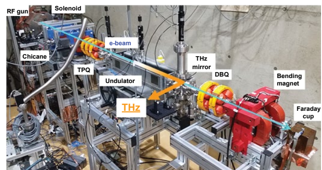
Figure 5: Beam line of the compact terahertz radiation source at Kyoto U.
