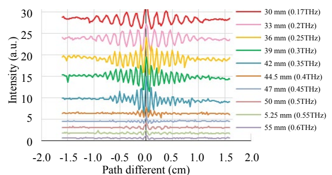
Figure 12: Measured interferograms by the Michelson interferometer for the compressed bunch with the different undulator gaps.
