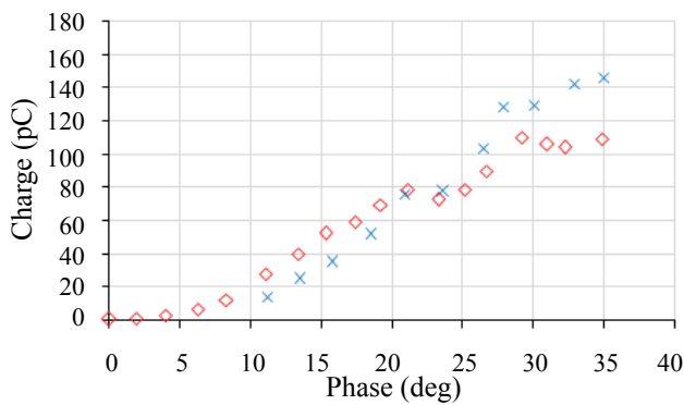
Figure 10: Measured bunch charge as a function of the laser injection phase at the undulator gap of 30 mm (square marks: compressed bunch, cross marks: uncompressed bunch).
