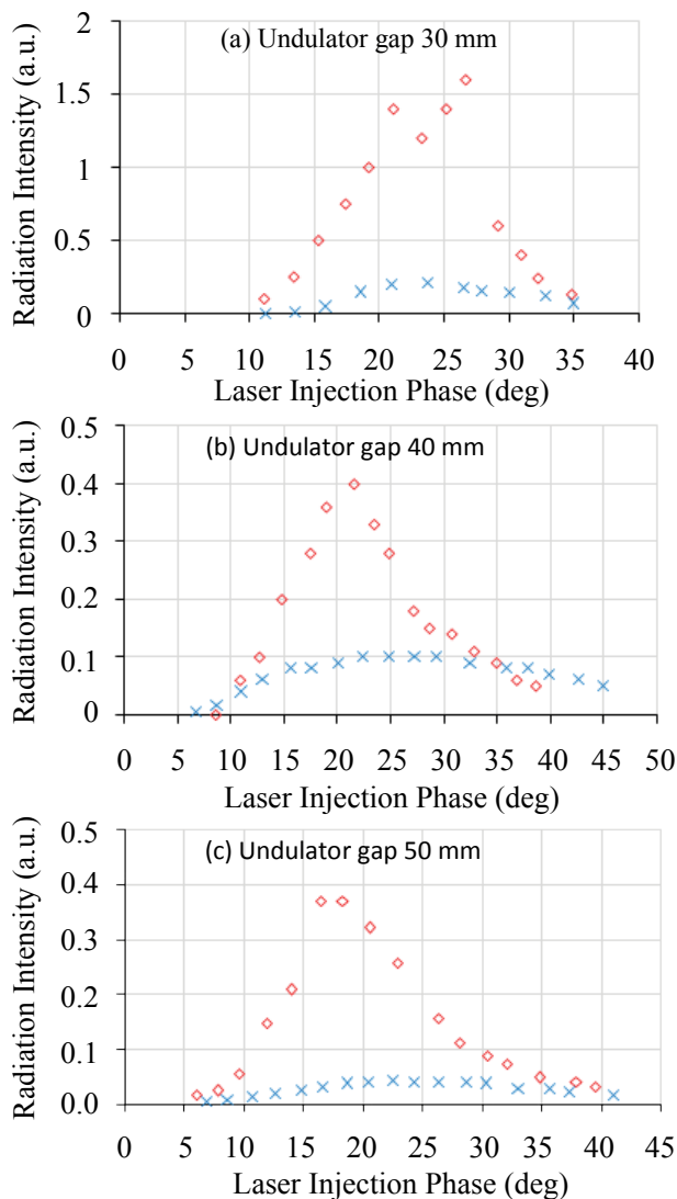
Figure 11: CUR intensity dependence on the laser injection phase at the undulator gap of a) 30 mm; b) 40 mm and c) 50 mm (square marks: compressed bunch, cross marks: uncompressed bunch).
