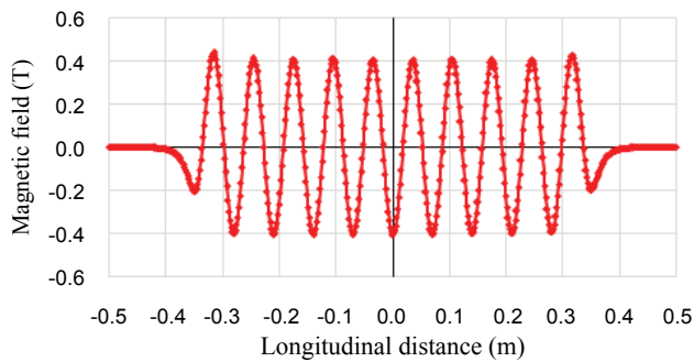
Figure 3: Measured transverse magnetic field at the center between poles at the undulator gap of 30 mm.
