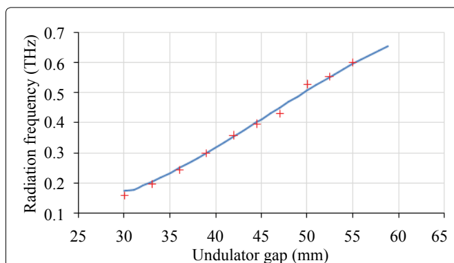
Figure 14: Central frequency of the CUR by calculation (solid line) and measurement (cross mark).
