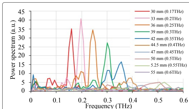
Figure 13: Power spectrum of the CUR for the different undulator gaps 30 to 55 mm. The frequencies in the bracket of the legend are the calculated radiation frequency.
