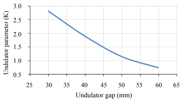
Figure 4: Undulator parameter ( K ) as a function of undulator gap calculated from the measured magnetic field.
