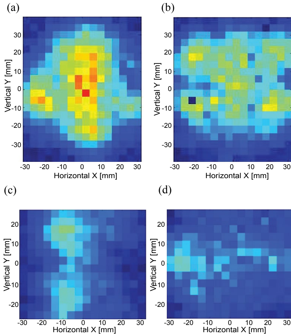
Figure 9: Spatial distributions of the CUR of the compressed bunch at the undulator gap of a) 30 mm; b) 35 mm; c) 180 mm and the uncompressed bunch at the undulator gap of d) 30 mm.
