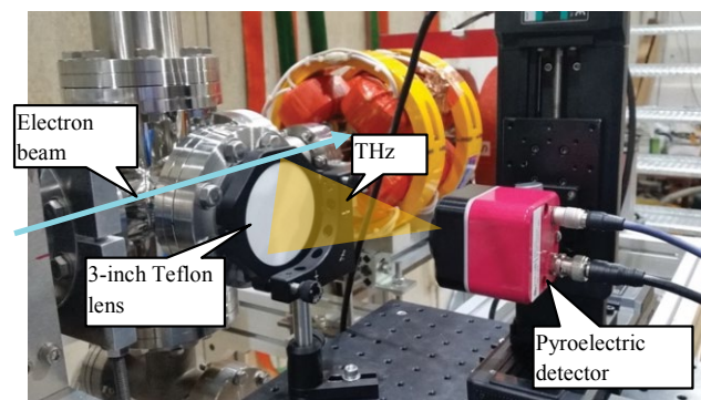
Figure 7: Total intensity measurement of the undulator radiation.
