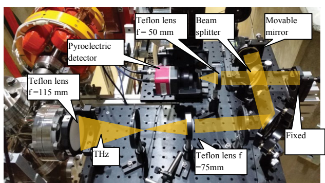
Figure 8: Set up of the Michelson interferometer for the power spectrum measurement.
