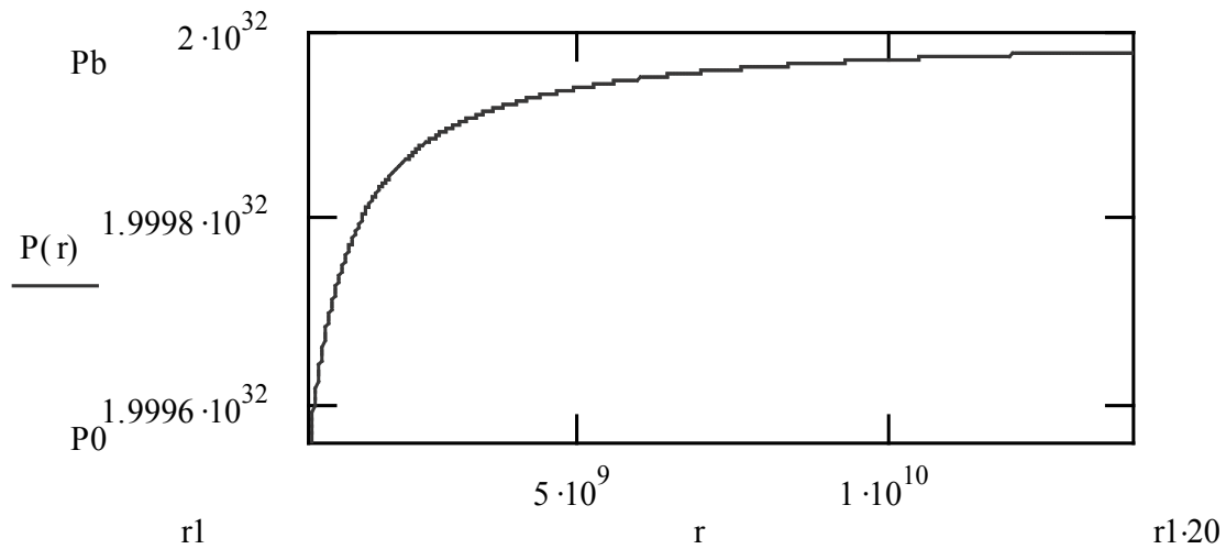
Figure 2: Radial distribution of ether pressure for the Sun.
