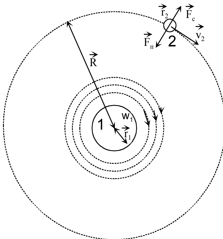
Figure 1: Two-dimensional model of the gravitational interaction between the two bodies.
